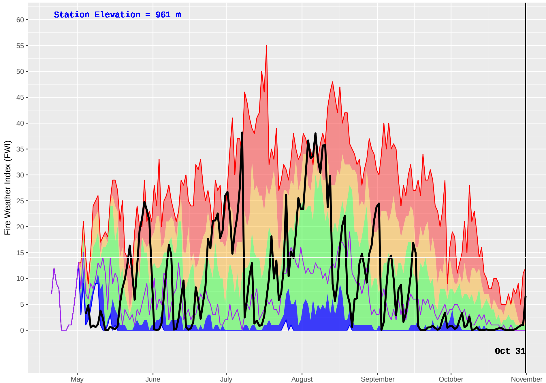
HOLY CROSS 2 (654) : Historical (1998–2016) and Current (2017) Noon Fire Weather Index (FWI)
