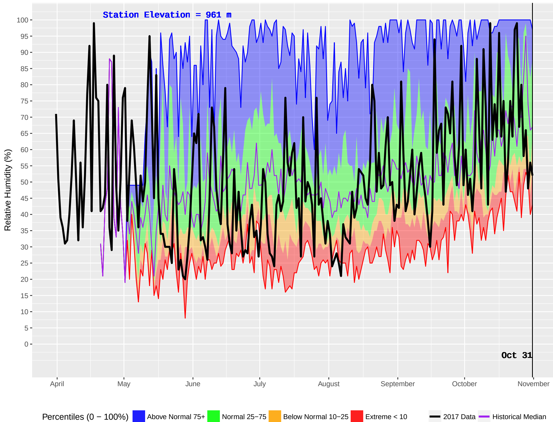
HOLY CROSS 2 (654) : Historical (1998–2016) and Current (2017) Noon Relative Humidity
