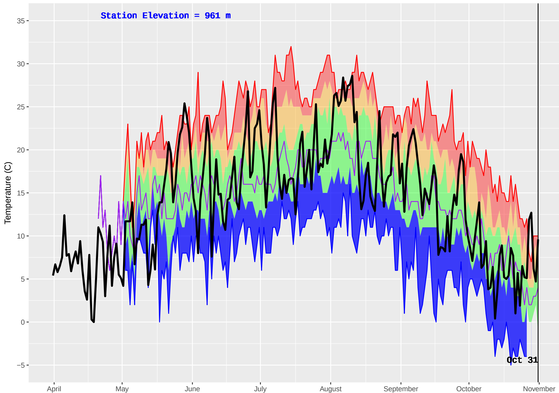
HOLY CROSS 2 (654) : Historical (1998–2016) and Current (2017) Noon Temperature
