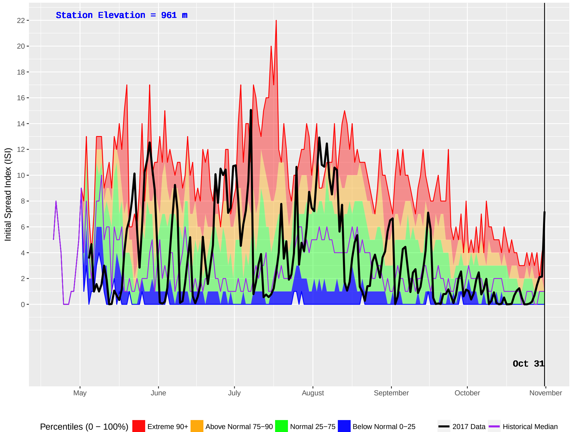
HOLY CROSS 2 (654) : Historical (1998–2016) and Current (2017) Noon Initial Spread Index (ISI)
