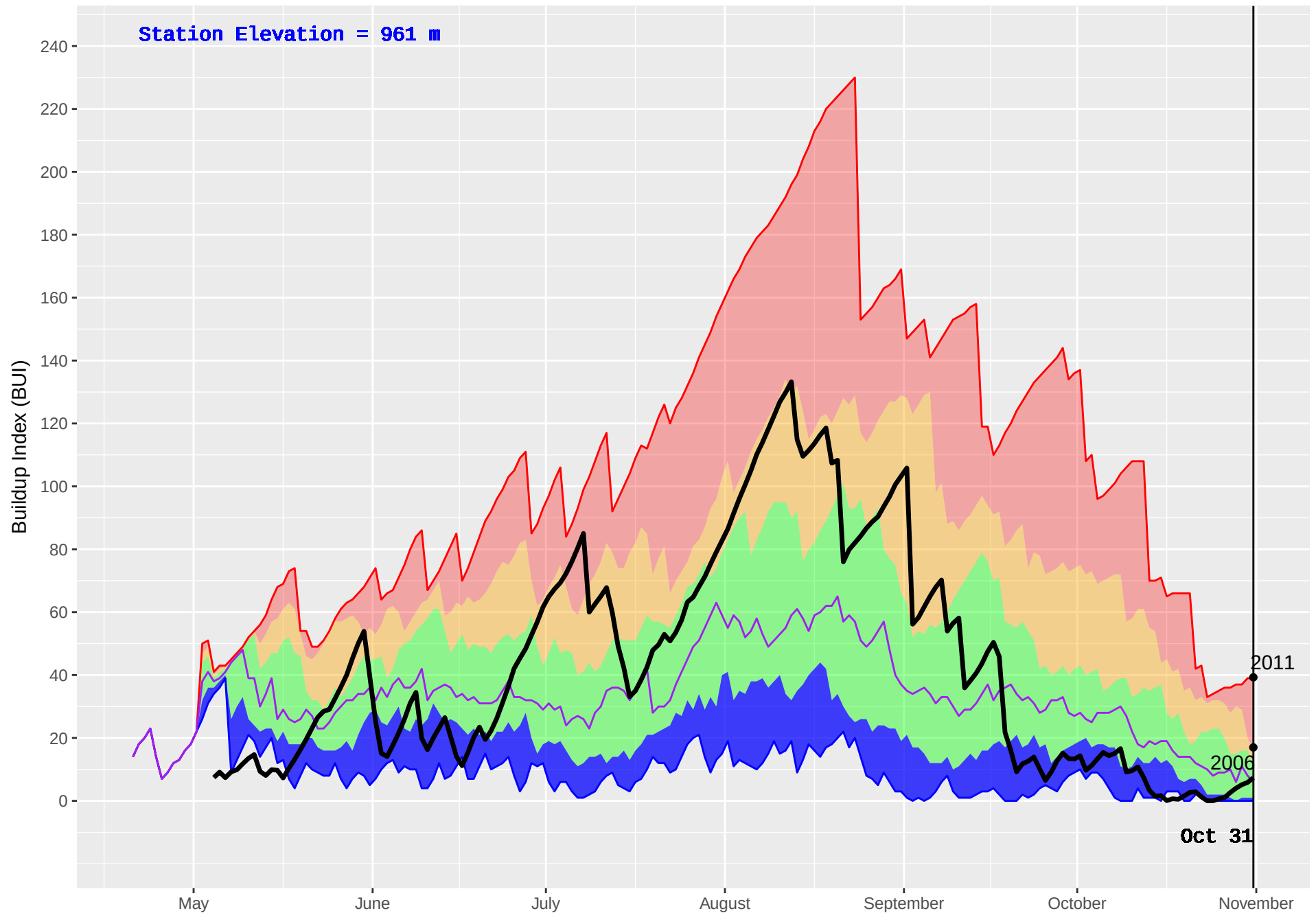
HOLY CROSS 2 (654) : Historical (1998–2016) and Current (2017) Noon Buildup Index (BUI)
